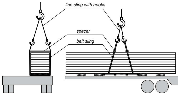
Fig. 10 Unloading of packages up to: - 6,5 m long for sandwich panels with PIR core - 7,5 m long for sandwich panels with mineral wool core
