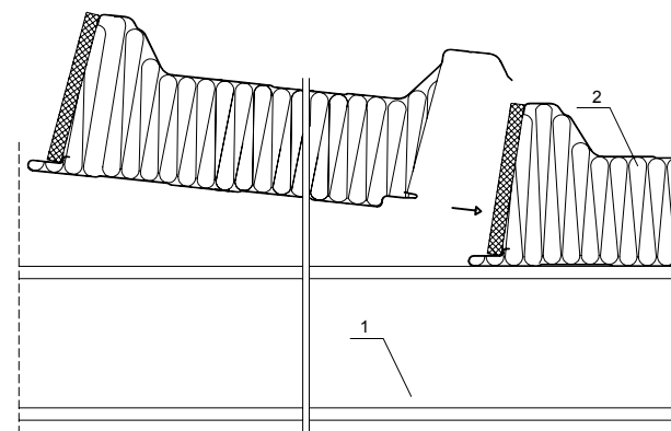
Pic. 8 and 9. Assembly of roof panels.
