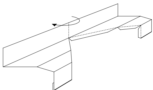
Fig. 18. External plinth corner.
