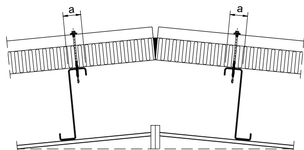
Fig. 21. Extreme supports a \geq 40 mm.
