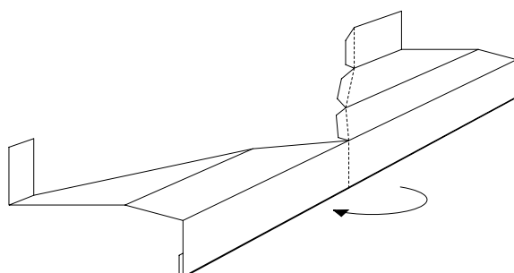
Fig.19. Plinth flashing external corner.
