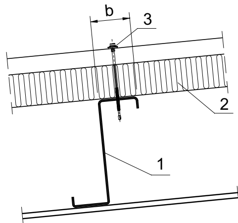
Fig. 20. Intermediate supports b \geq 60 mm, where:
