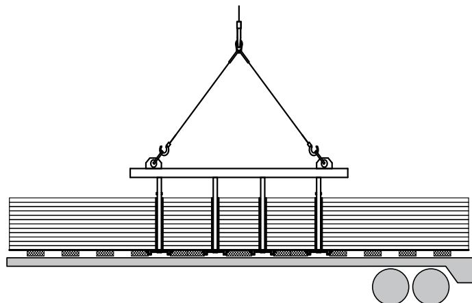
Fig. 11 Unloading of packages longer than: - 6,5 m for sandwich panels with PIR core - 7,5 m for sandwich panels with mineral wool core
